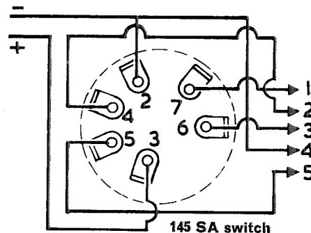
ALTERNATIVE SWITCHES INDICATING MOULDED TERMINAL CONNECTIONS
