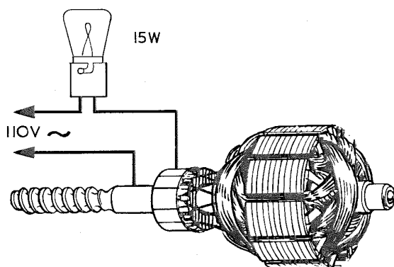
Fig. 4 Armature insulation test
