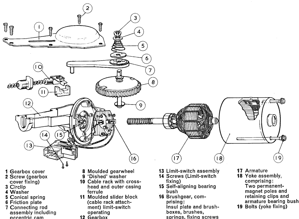
Fig. 1 Windshield Wiper Motor Model 16W (two speed)
