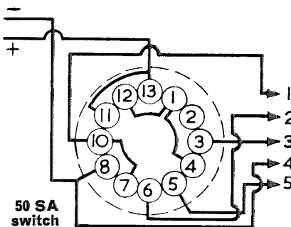
ALTERNATIVE SWITCHES INDICATING MOULDED TERMINAL CONNECTIONS
