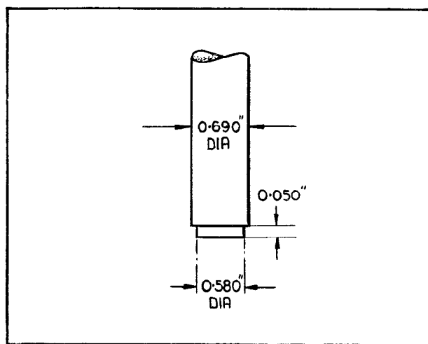
Fig. 7 Mandrel to expand oil seal
